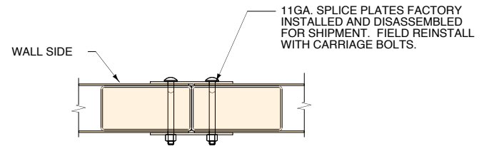
SPLICE PLATE DETAIL (IF REQUIRED)
